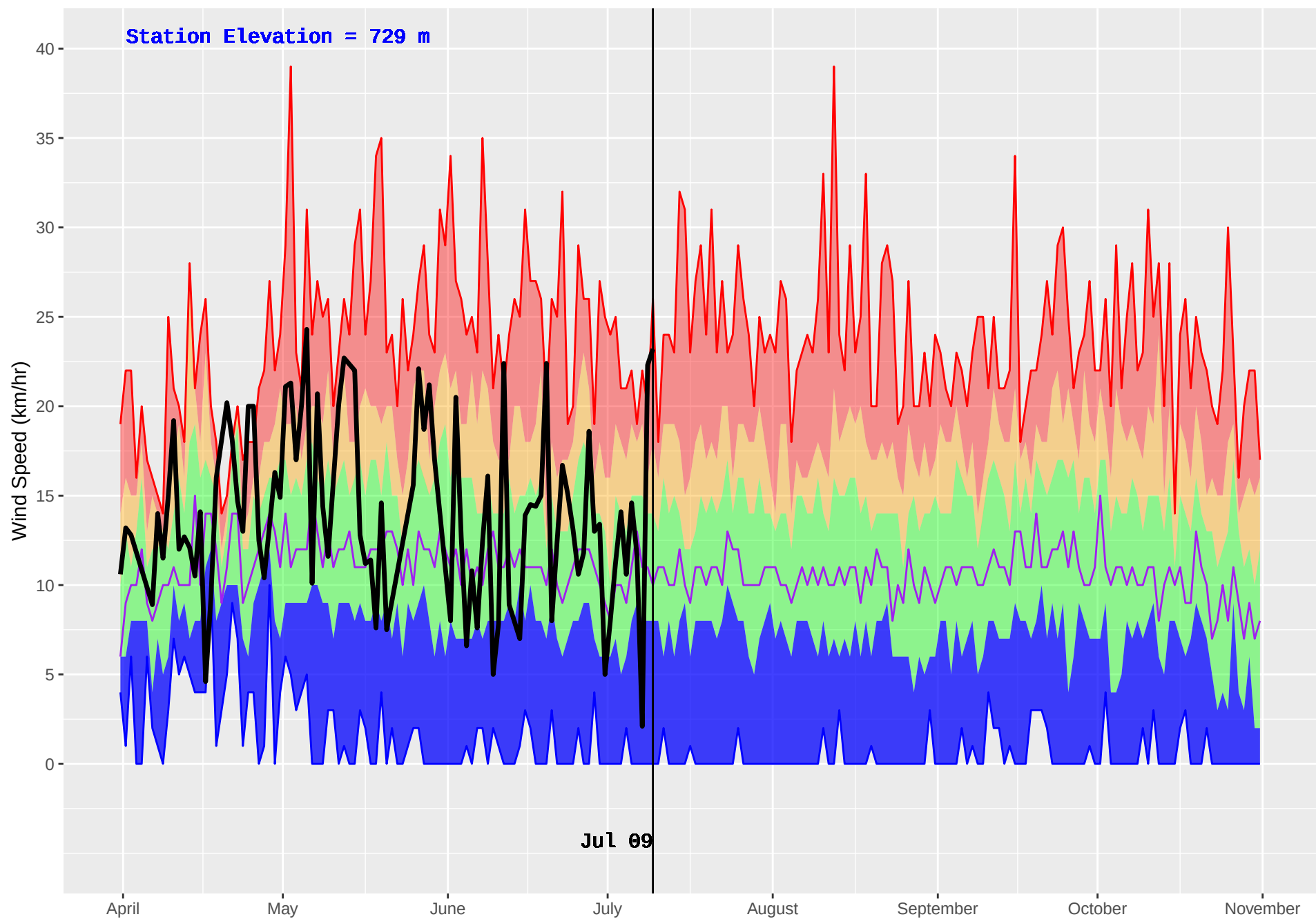
ATLIN (111) : Historical (1977–2016) and Current (2018) Daily Wind Speed
