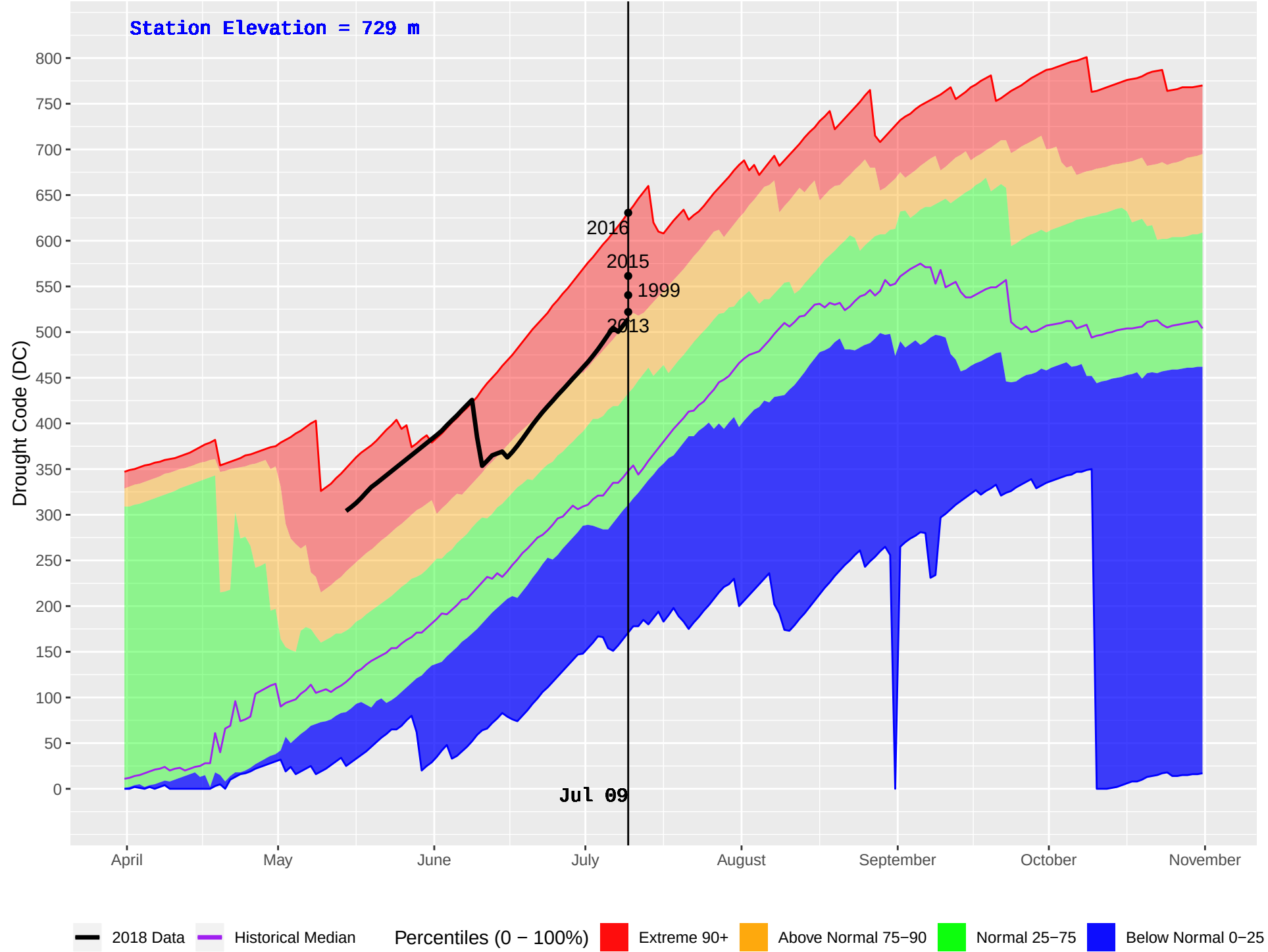
ATLIN (111) : Historical (1977–2016) and Current (2018) Daily Drought Code (DC)
