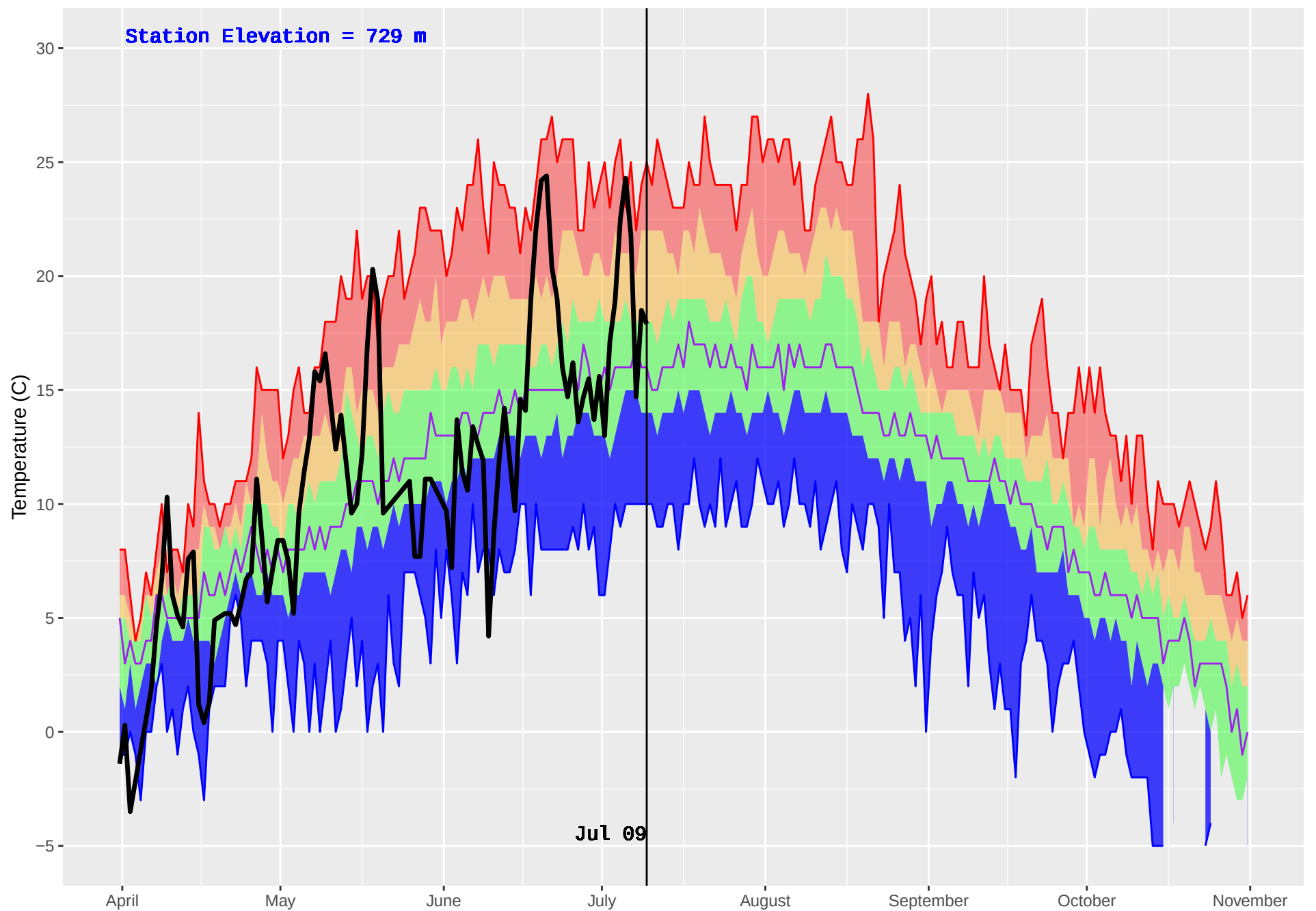
ATLIN (111) : Historical (1977–2016) and Current (2018) Daily Temperature
