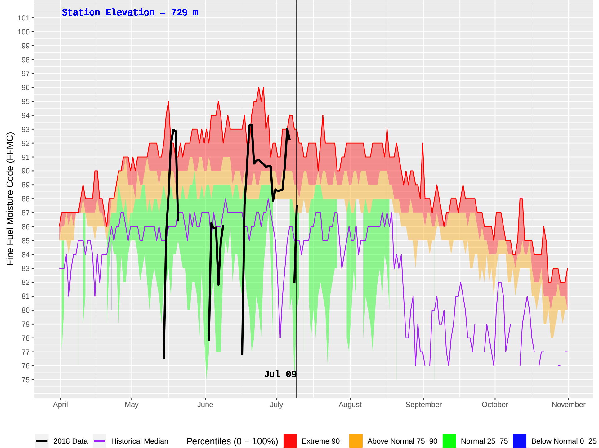
ATLIN (111) : Historical (1977–2016) and Current (2018) Daily Fine Fuel Moisture Code (FFMC)
