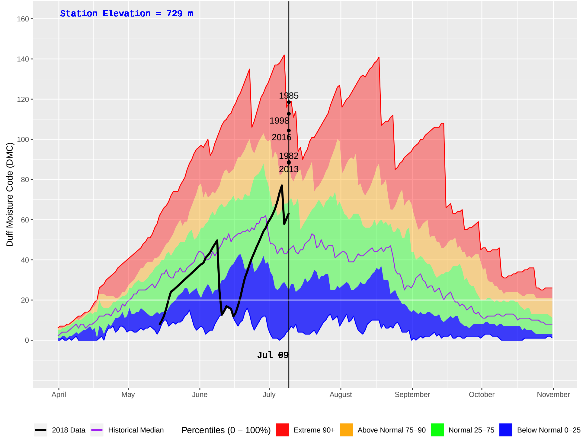
ATLIN (111) : Historical (1977–2016) and Current (2018) Daily Duff Moisture Code (DMC)
