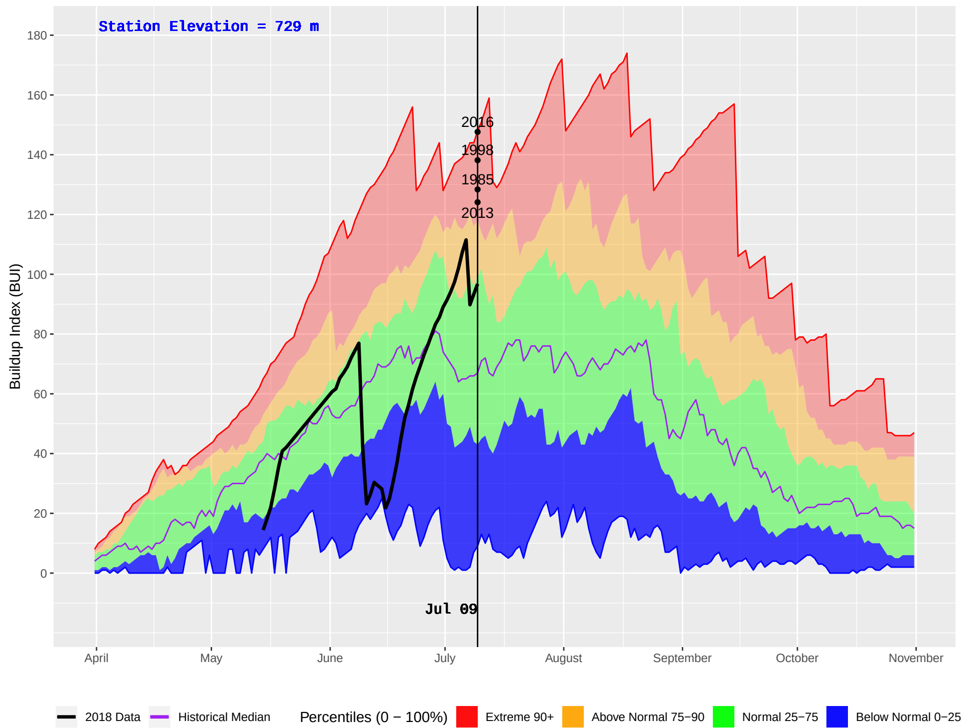
ATLIN (111) : Historical (1977–2016) and Current (2018) Daily Buildup Index (BUI)
