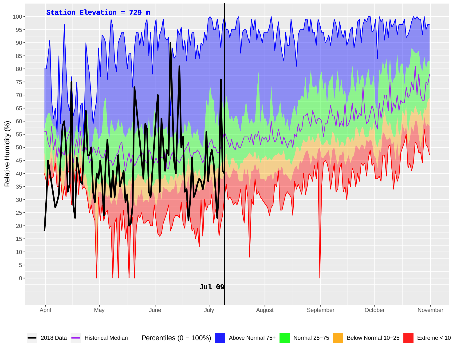
ATLIN (111) : Historical (1977–2016) and Current (2018) Daily Relative Humidity
