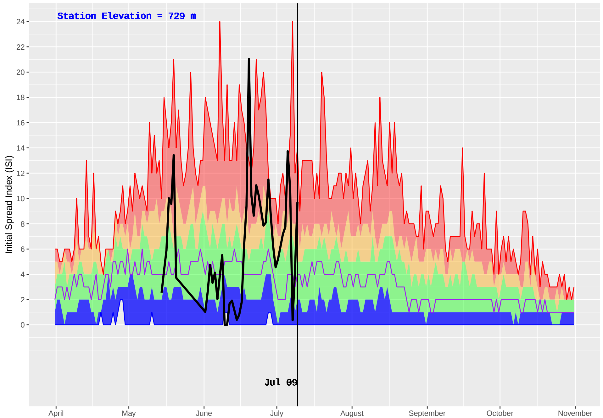
ATLIN (111) : Historical (1977–2016) and Current (2018) Daily Initial Spread Index (ISI)
