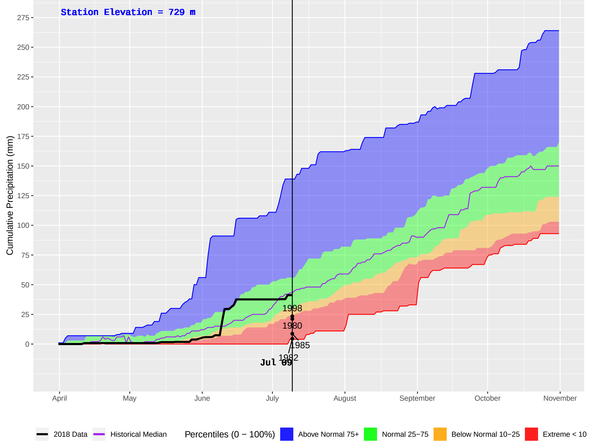
ATLIN (111) : Historical (1977–2016) and Current (2018) Daily Cumulative Precipitation
